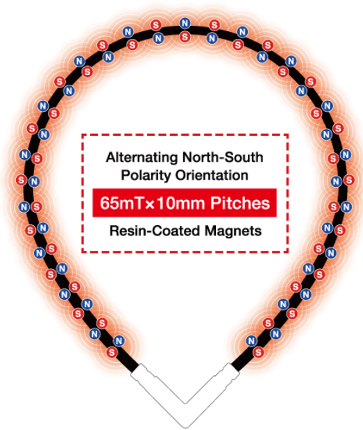
Magnet layout diagram
